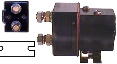
138684 Solenoid 12 V, 100 A, Coil bolt M8, No./ terminals 4 Silver contact.
