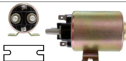
333153 Solenoid Manufacturer: Bosch Replacing: 19024761 12 V, 150 A, Intermittent load 800 Amp., OD 51.75, Coil bolt M8, Seconds 5, No./ terminals 4 Silver contact. Insulated return. Alternative no.: 131373, 131373Z
