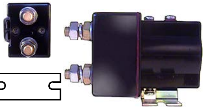
138685 Solenoid 24 V, 100 A, Coil bolt M8, No./ terminals 4 Silver contact.
