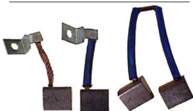
PSX122-123-124 Brush Set Replacing: 182073 12 V, Length 15.10, Height 12.45, Thickness 4.50/8.90
