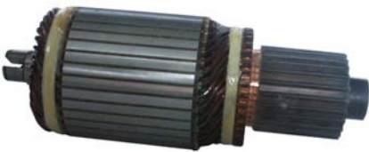
135760# Armature 12 V, 3 kW, Shaft length 221.00, Core thickness 81.75
