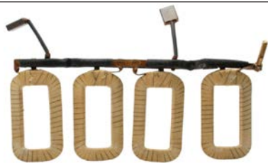
135200 Field Coil
