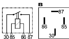
160652 6 V. 20 Amp. 4 terminals.
