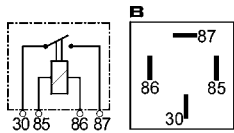
160080 A 12 V. 30 Amp. 4 terminals.
