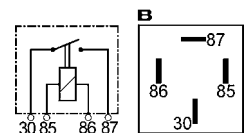
160240 A 24 V. 30 Amp. 4 terminals. W/ two 6.3 mm. and two 9.5 mm. terminals (terminals 30 and 87).
