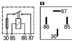
160473 A 24 V. 15 Amp. 4 terminals. W/ insertable ATO-blade fuse.
