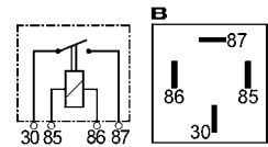
160239 A 12 V. 70 Amp. 4 terminals. W/ two 6.3 mm. and two 9.5 mm. terminals (terminals 30 and 87).
