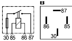
160155 A 12 V. 15 Amp. 4 terminals. W/ insertable ATO-blade fuse.
