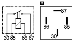
160082 A 24 V. 20 Amp. 4 terminals.
