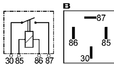
160307 A Std pkg 10 As Cargo 160082, but w/o bracket. 24 V. 20 Amp. 4 terminals.
