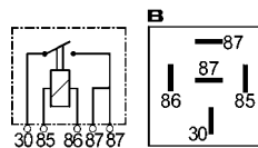
160266 A 24 V. 20 Amp. 5 terminals
